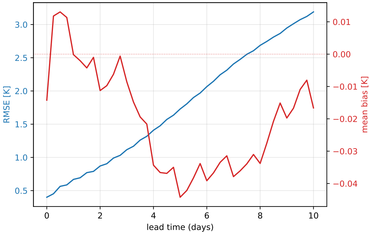
ERA5 2023 — 900 hPa temperature (global, mean of 31 daily inits)
