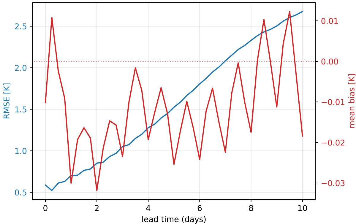
ERA5 2023 — 1000 hPa temperature (global, mean of 31 daily inits)
