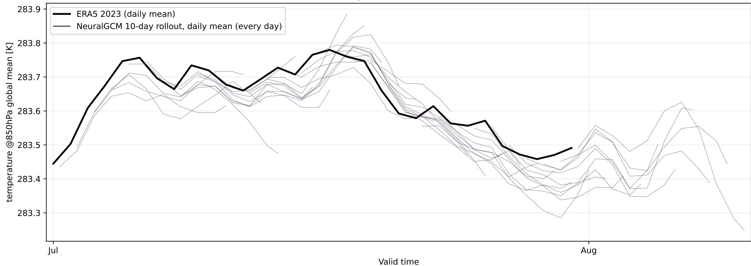
Global-mean temperature at 850 hPa — ERA5 2023
