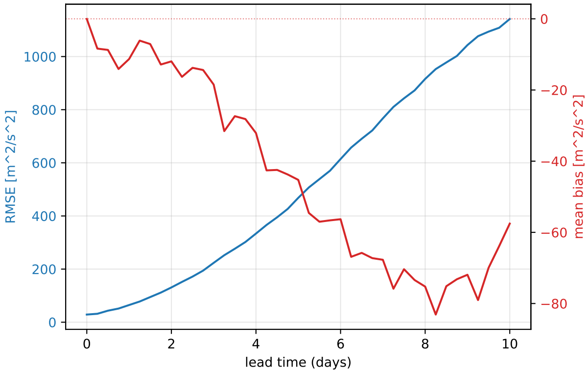
ERA5 2026 — 500 hPa geopotential (europe, mean of 181 daily inits)
