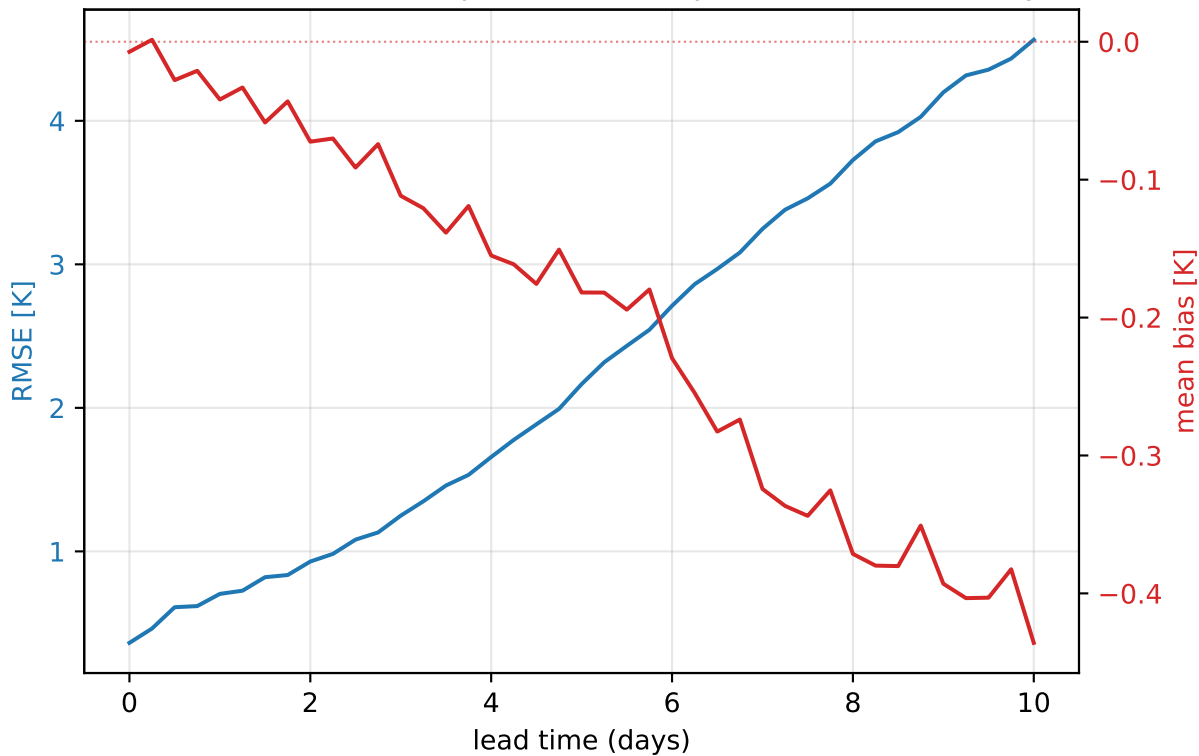
ERA5 2026 — 850 hPa temperature (europe, mean of 181 daily inits)
