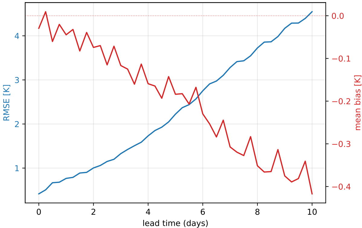
ERA5 2026 — 900 hPa temperature (europe, mean of 181 daily inits)
