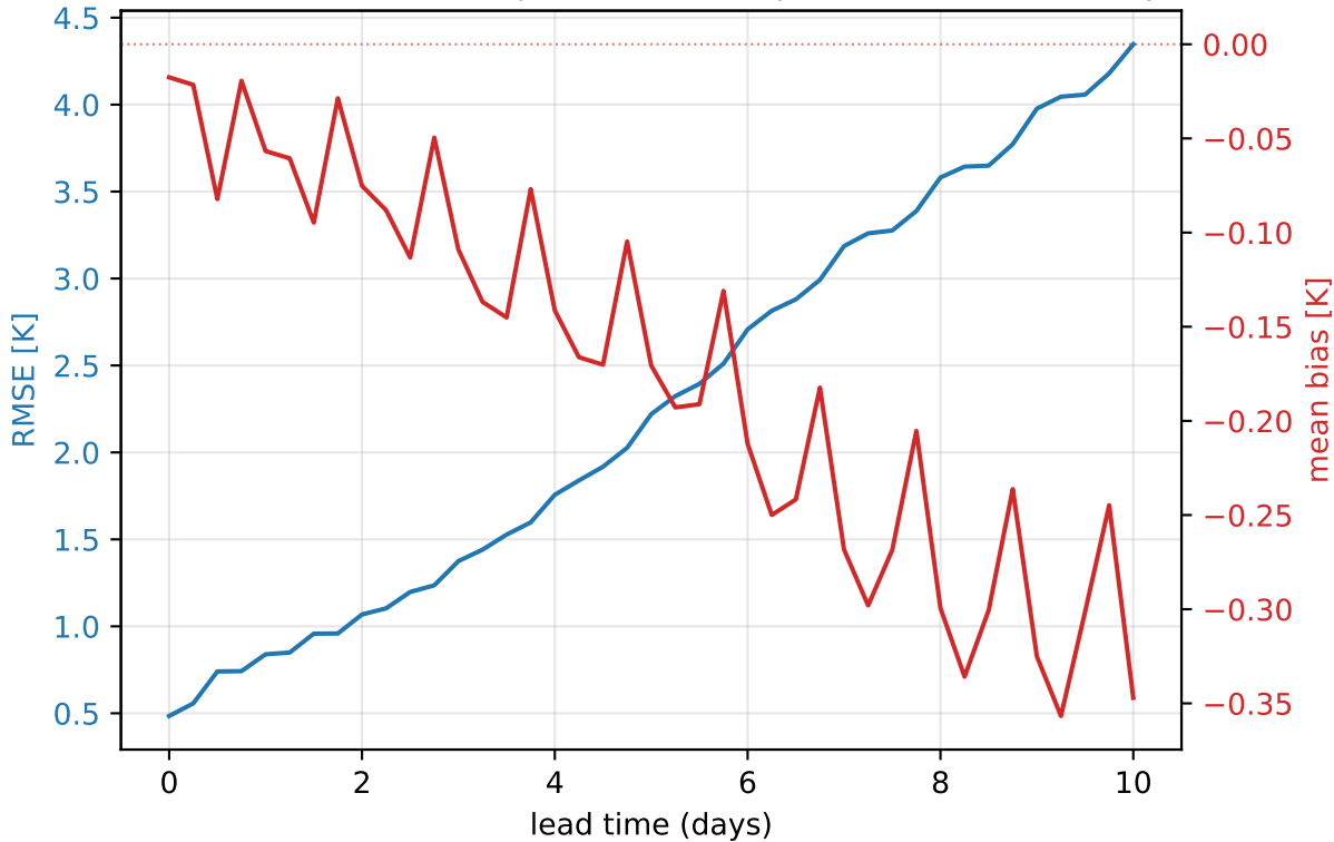
ERA5 2026 — 950 hPa temperature (europe, mean of 181 daily inits)
