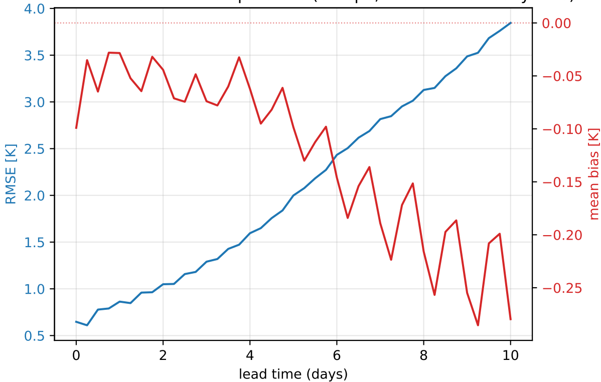
ERA5 2026 — 1000 hPa temperature (europe, mean of 181 daily inits)
