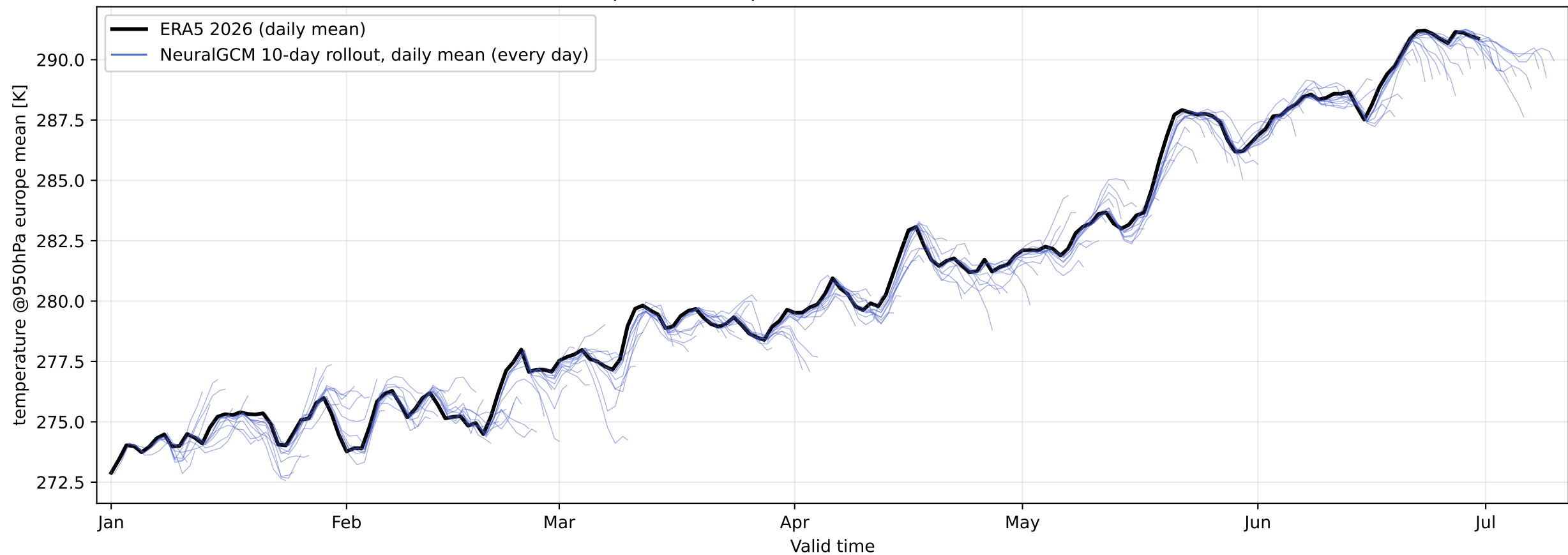
Europe-mean temperature at 950 hPa — ERA5 2026
