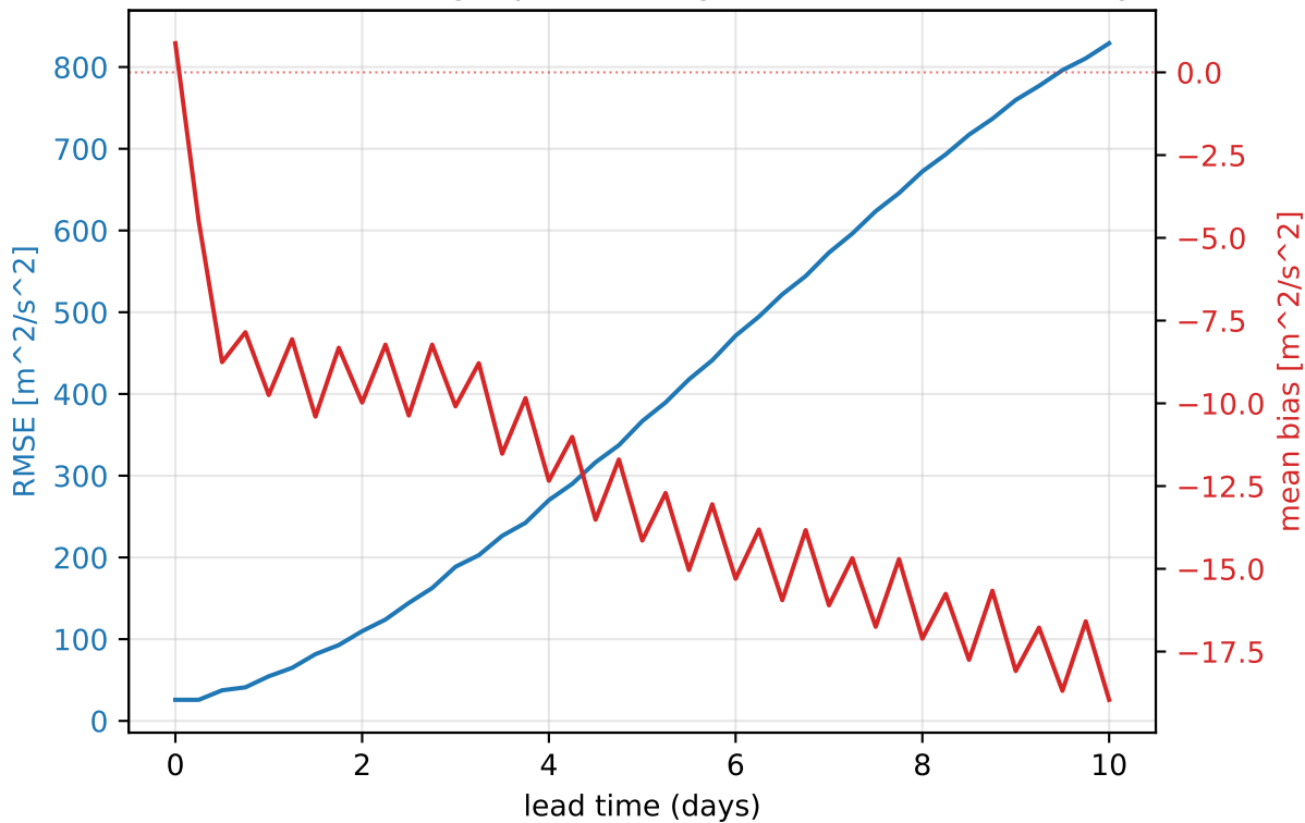
ERA5 2026 — 500 hPa geopotential (global, mean of 181 daily inits)
