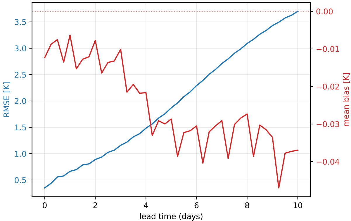
ERA5 2026 — 850 hPa temperature (global, mean of 181 daily inits)
