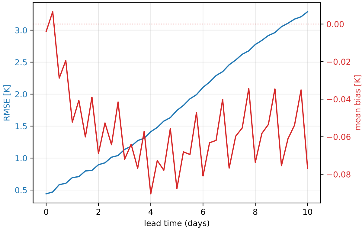
ERA5 2026 — 950 hPa temperature (global, mean of 181 daily inits)
