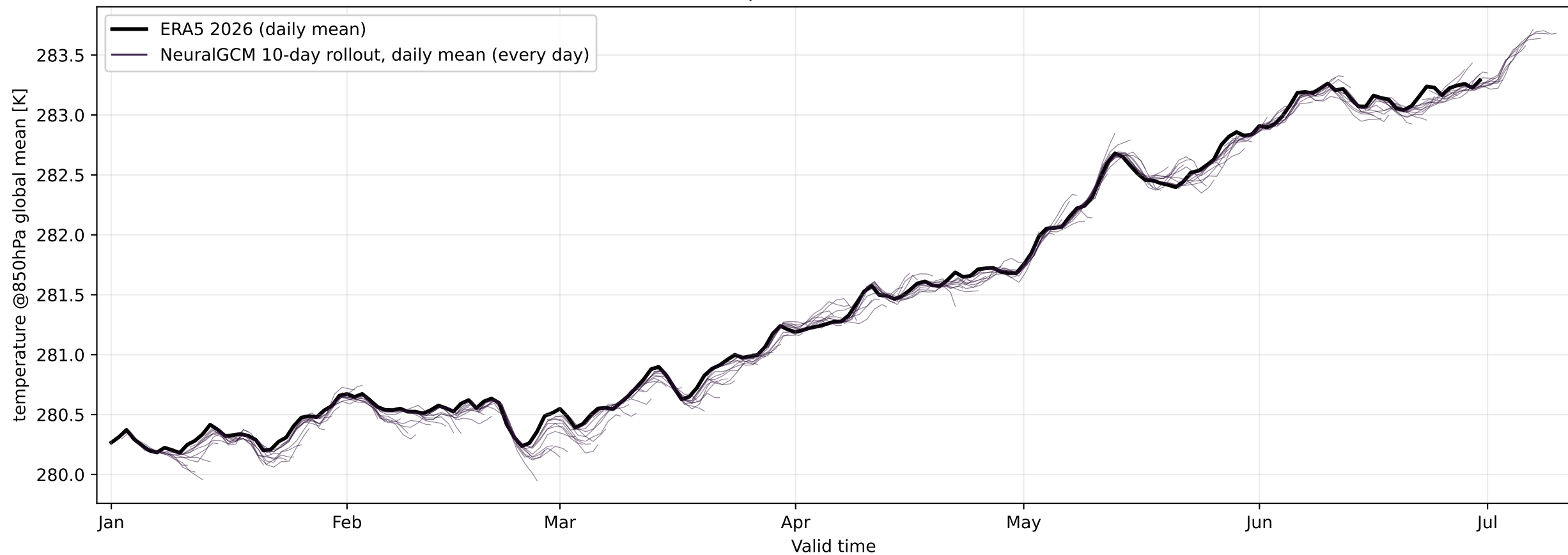
Global-mean temperature at 850 hPa — ERA5 2026
