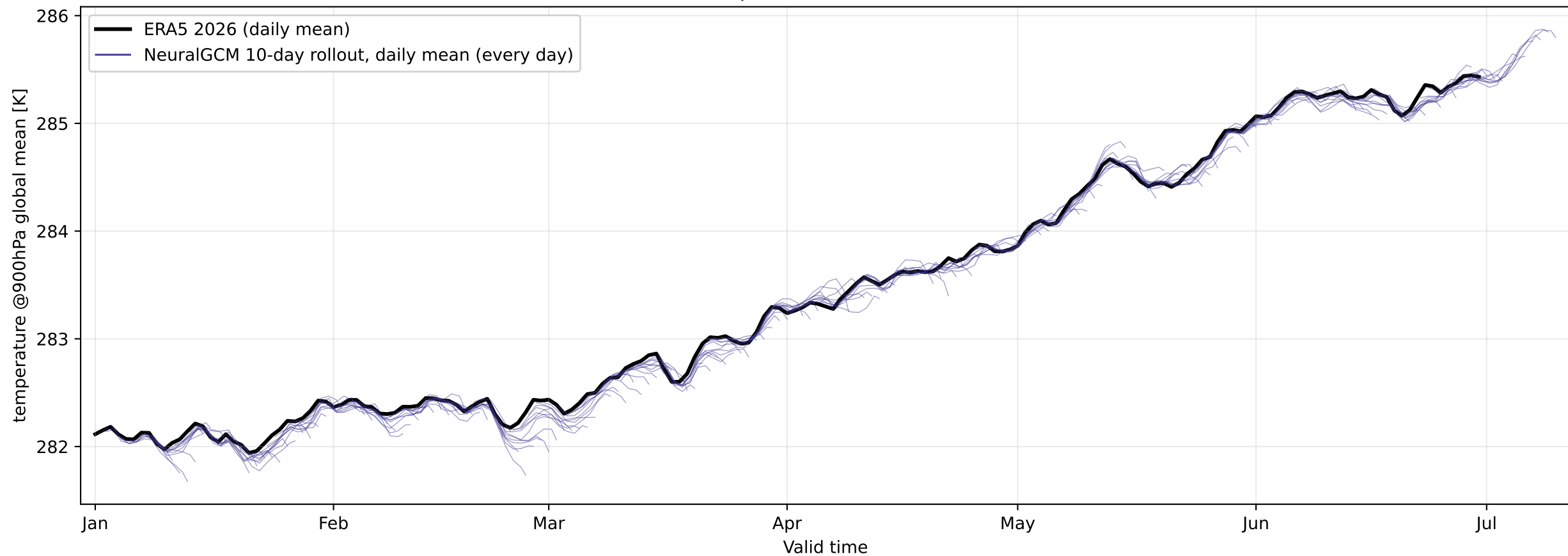
Global-mean temperature at 900 hPa — ERA5 2026
