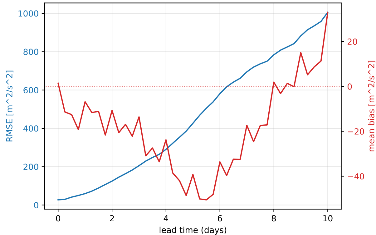
ERA5 2026 — 500 hPa geopotential (europe, mean of 31 daily inits)
