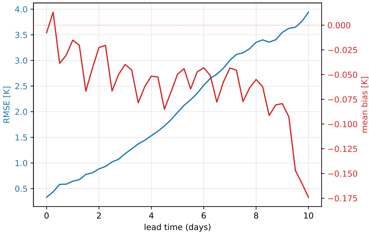
ERA5 2026 — 850 hPa temperature (europe, mean of 31 daily inits)
