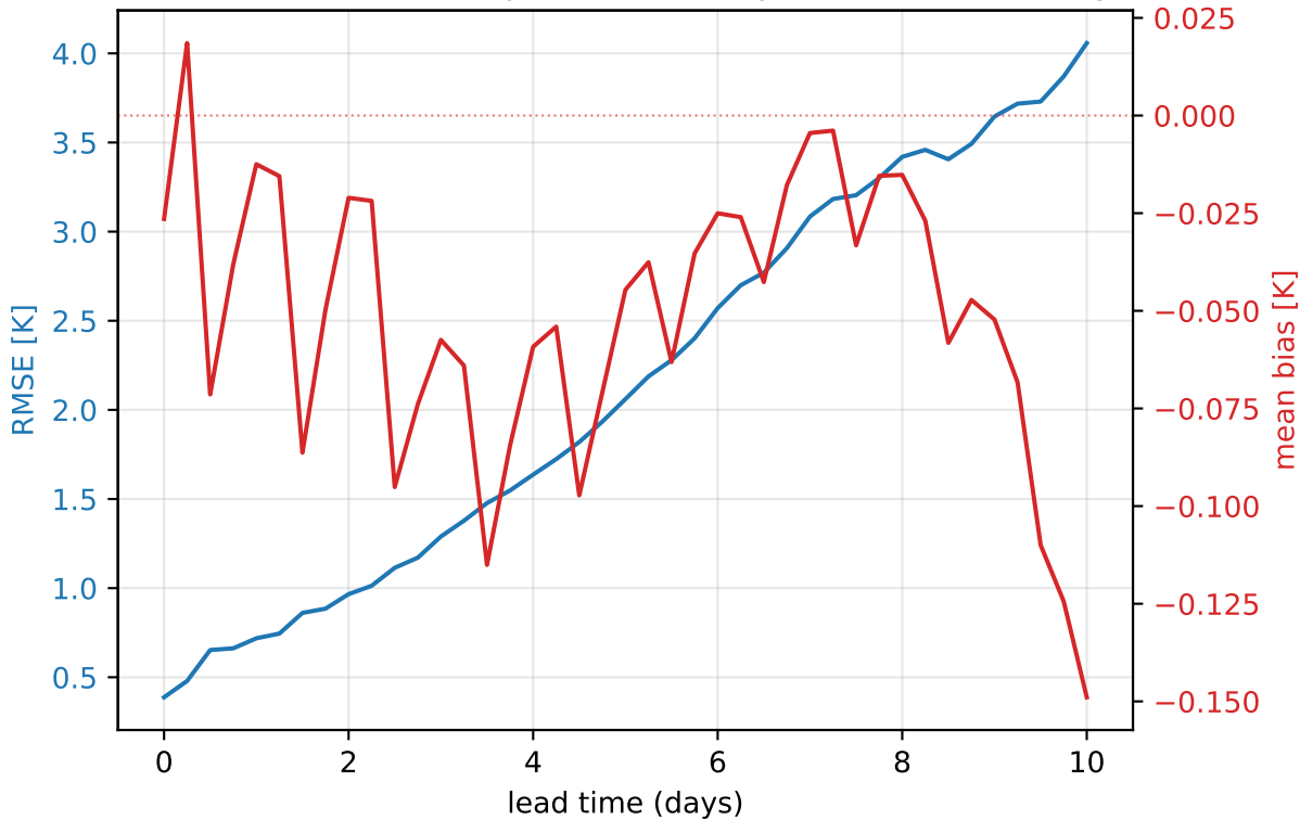
ERA5 2026 — 900 hPa temperature (europe, mean of 31 daily inits)
