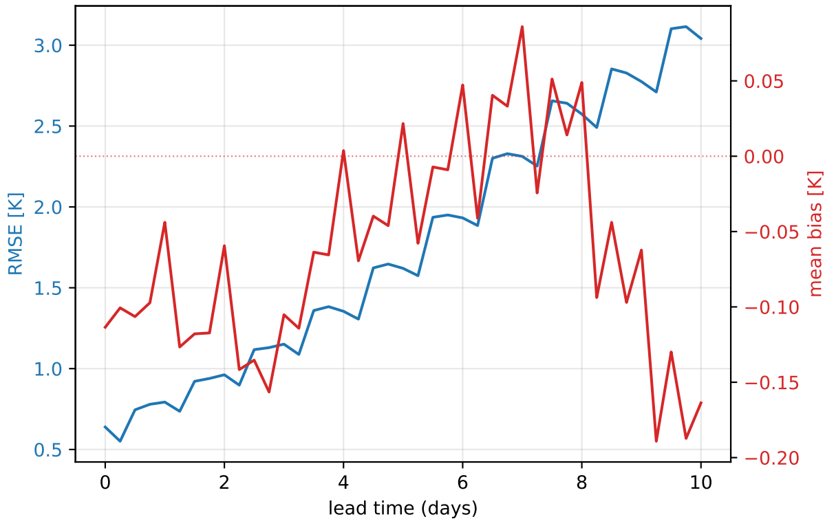
ERA5 2026 — 1000 hPa temperature (europe, mean of 31 daily inits)
