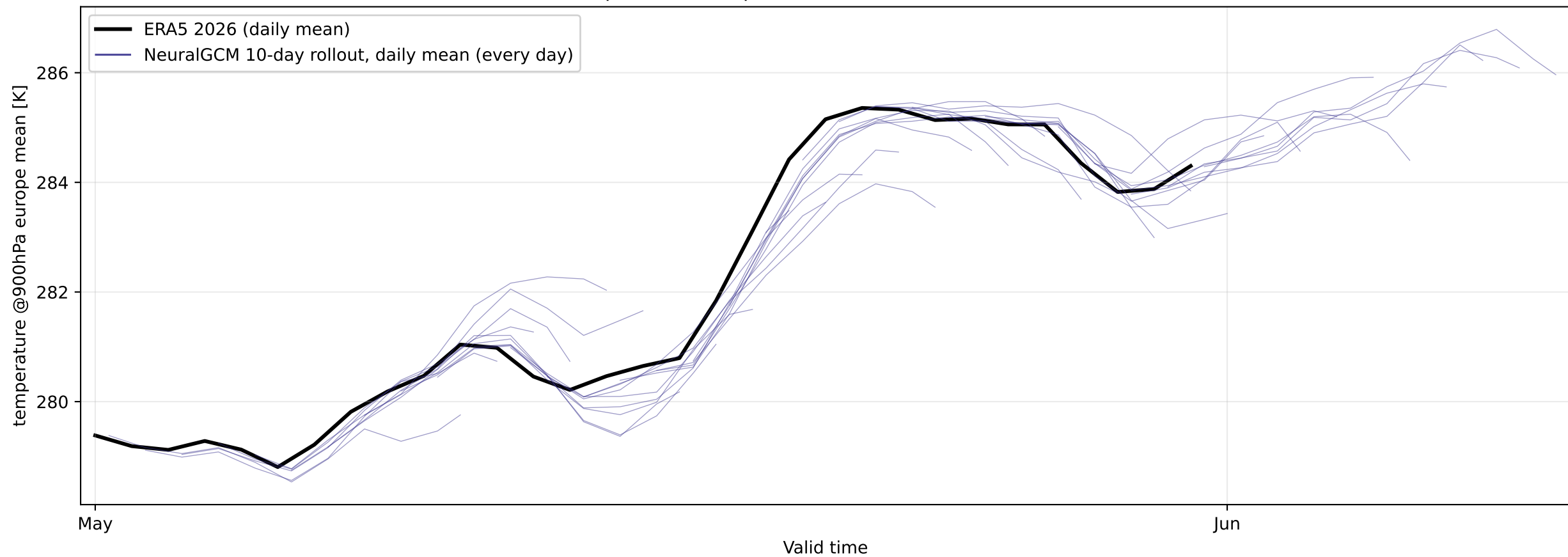
Europe-mean temperature at 900 hPa — ERA5 2026
