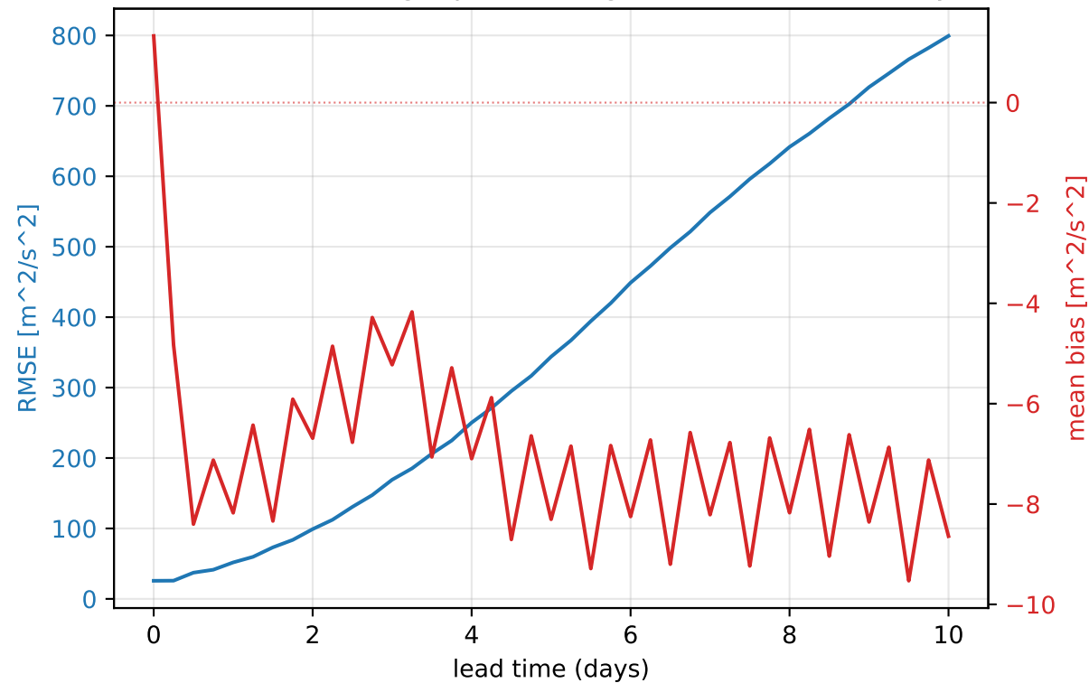
ERA5 2026 — 500 hPa geopotential (global, mean of 31 daily inits)
