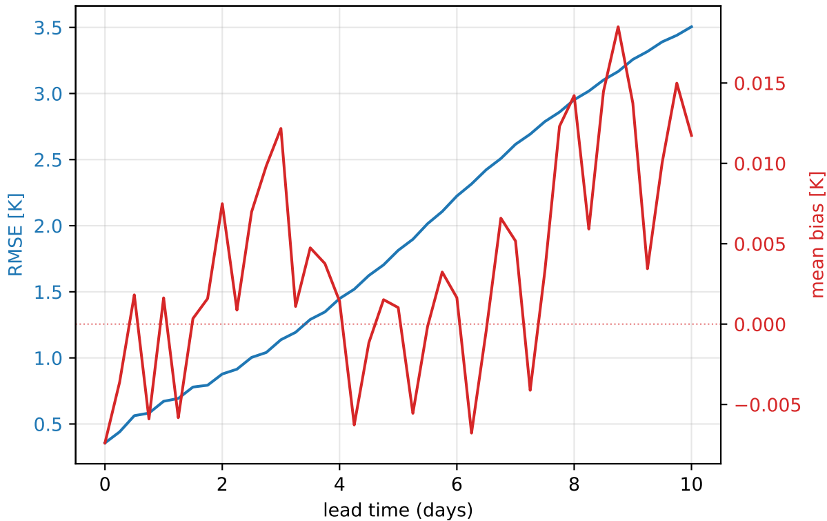
ERA5 2026 — 850 hPa temperature (global, mean of 31 daily inits)
