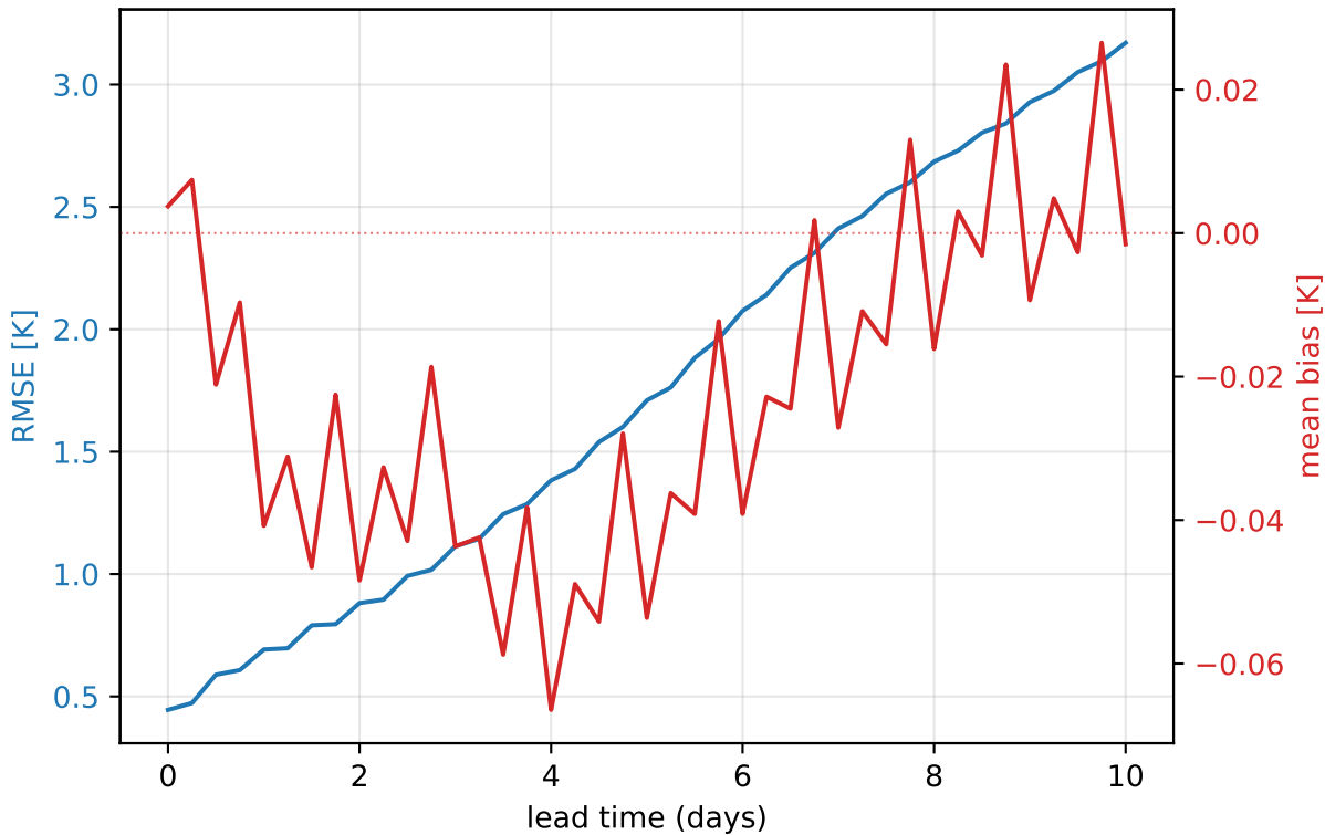
ERA5 2026 — 950 hPa temperature (global, mean of 31 daily inits)
