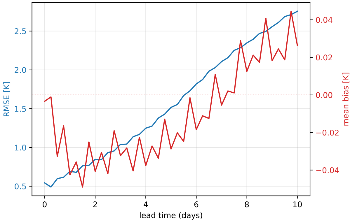
ERA5 2026 — 1000 hPa temperature (global, mean of 31 daily inits)
