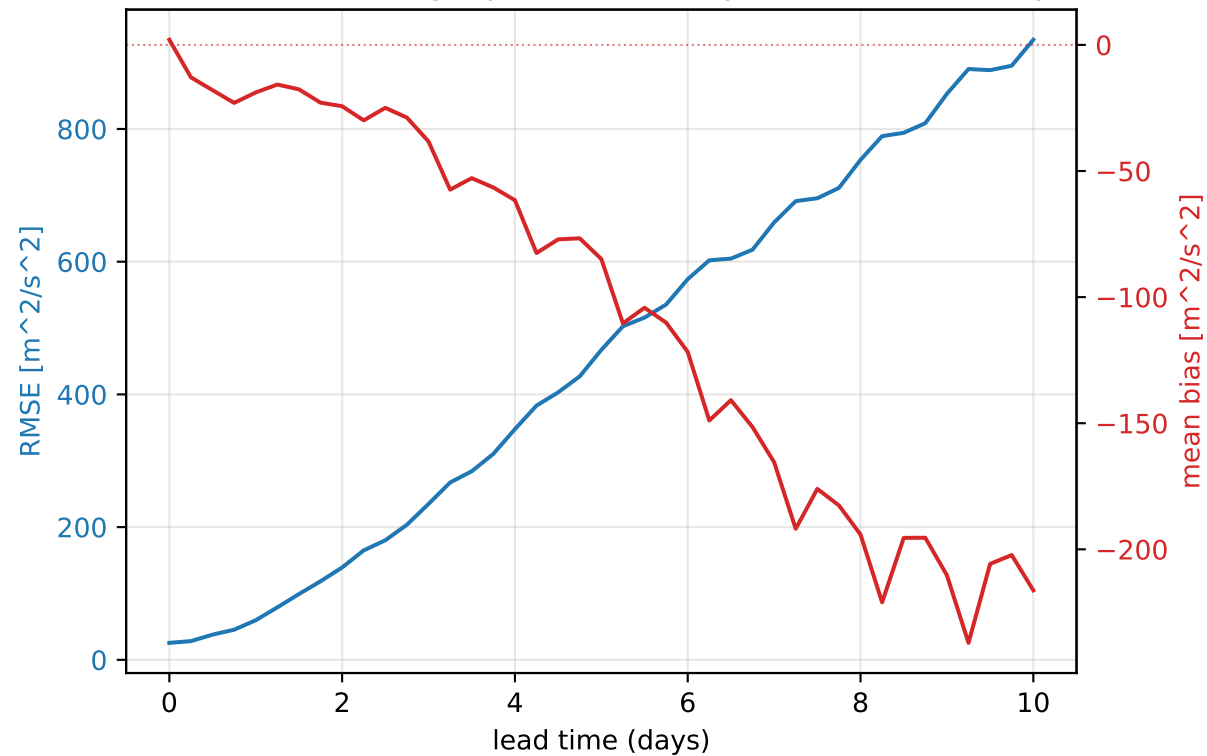
ERA5 2026 — 500 hPa geopotential (europe, mean of 30 daily inits)
