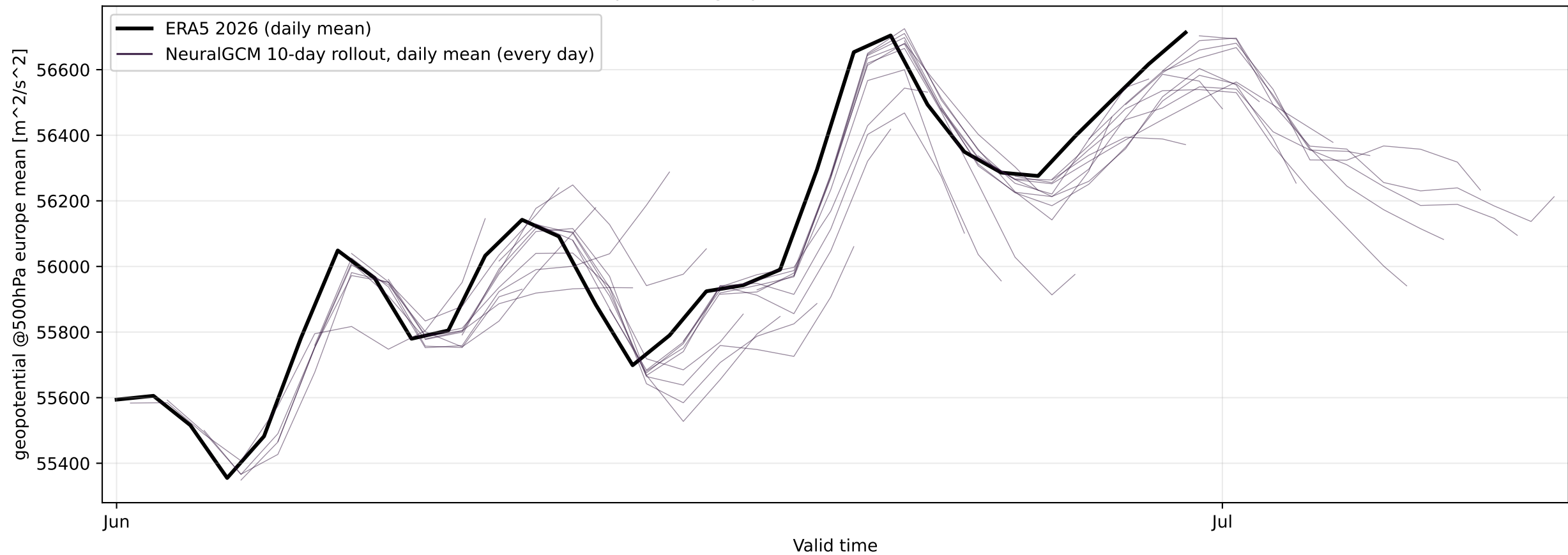
Europe-mean geopotential at 500 hPa — ERA5 2026
