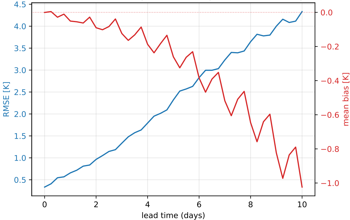
ERA5 2026 — 850 hPa temperature (europe, mean of 30 daily inits)
