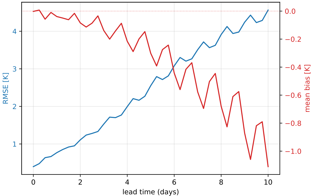
ERA5 2026 — 900 hPa temperature (europe, mean of 30 daily inits)
