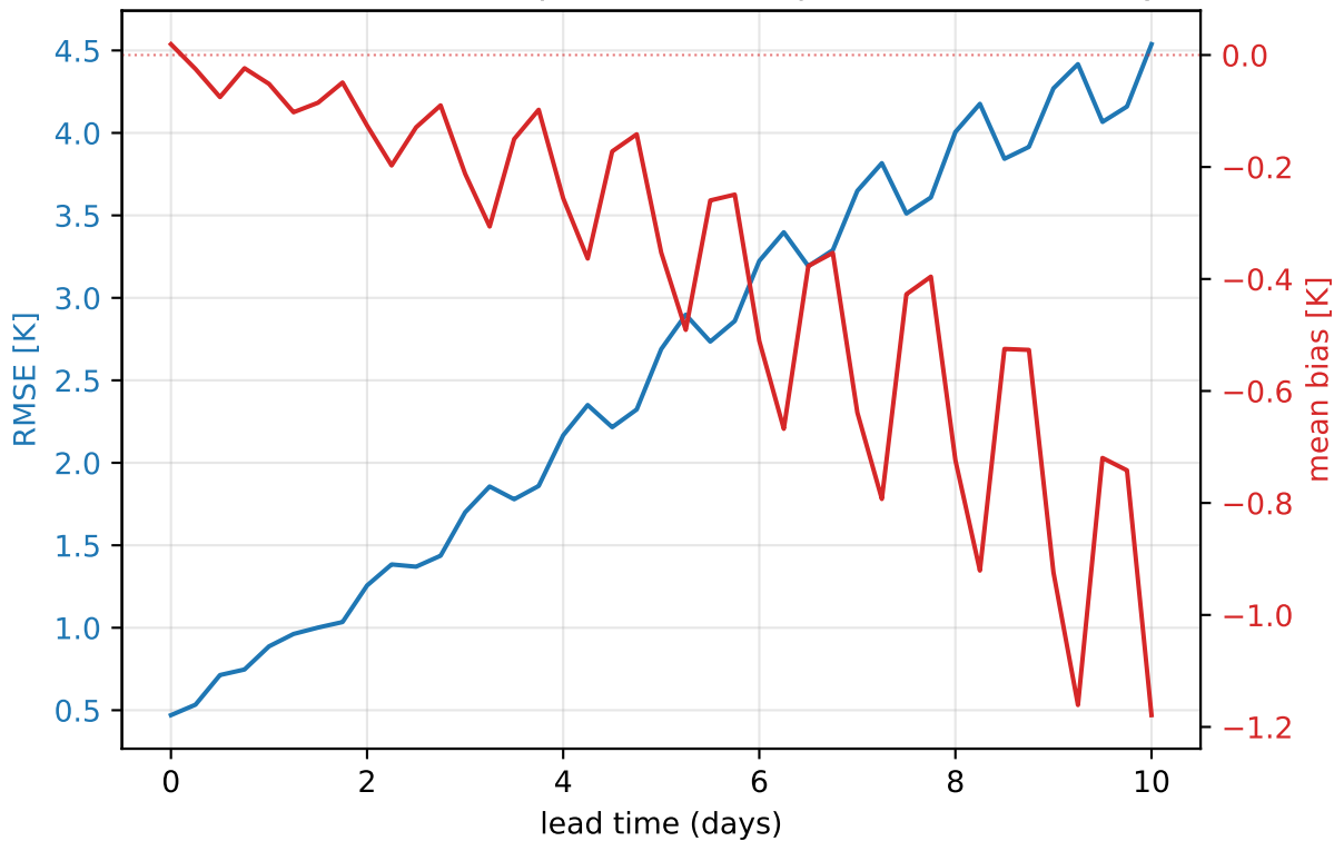
ERA5 2026 — 950 hPa temperature (europe, mean of 30 daily inits)
