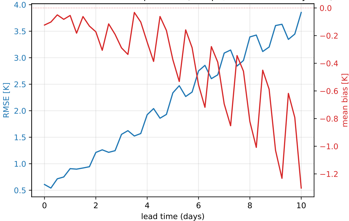
ERA5 2026 — 1000 hPa temperature (europe, mean of 30 daily inits)
