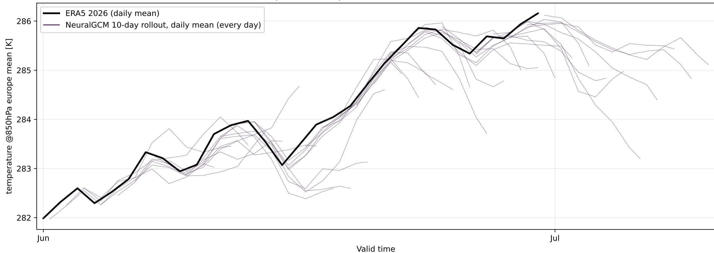
Europe-mean temperature at 850 hPa — ERA5 2026
