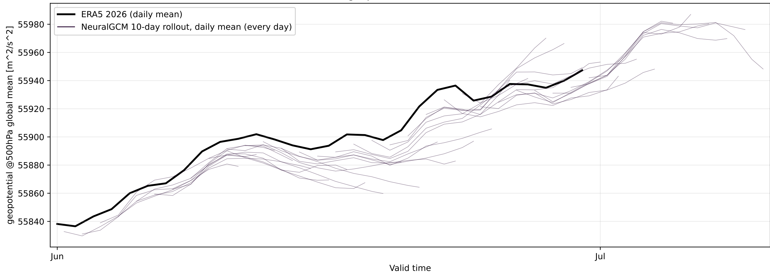
Global-mean geopotential at 500 hPa — ERA5 2026
