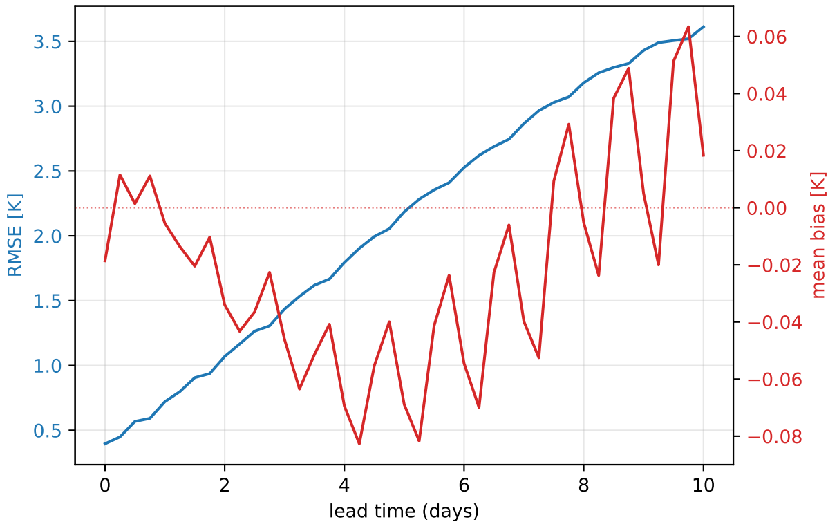
ERA5 2026 — 900 hPa temperature (global, mean of 30 daily inits)
