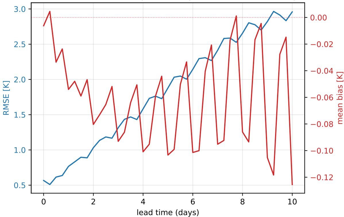
ERA5 2026 — 1000 hPa temperature (global, mean of 30 daily inits)
