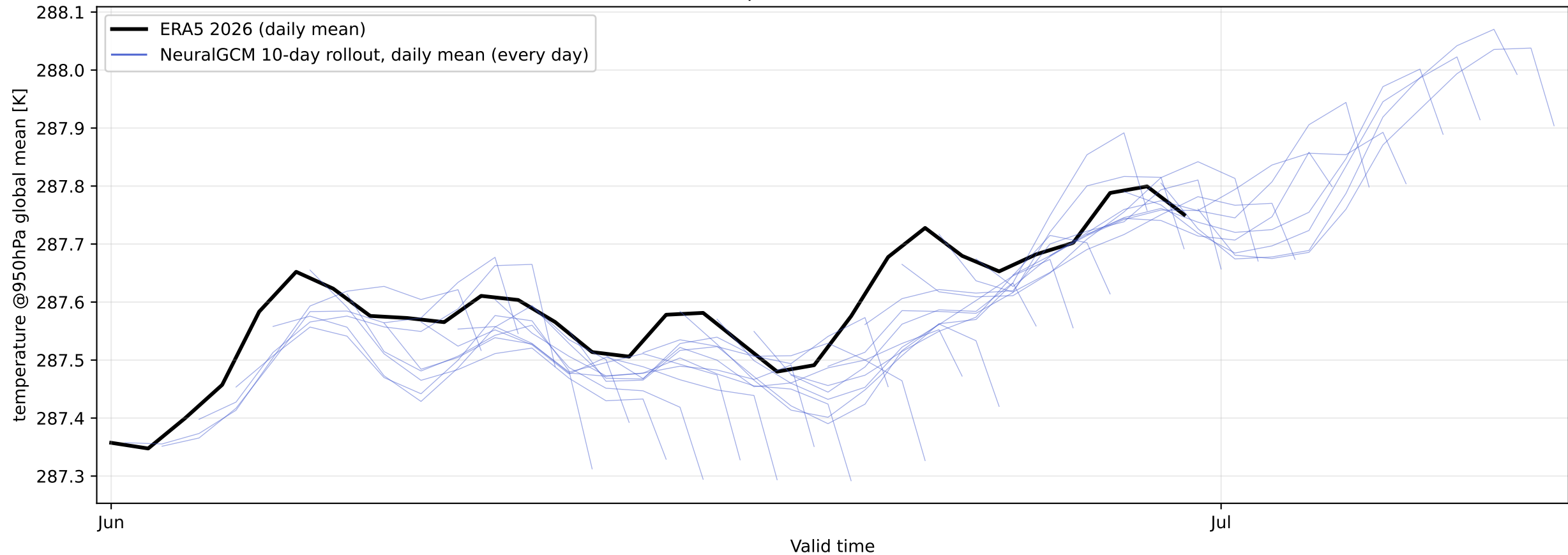
Global-mean temperature at 950 hPa — ERA5 2026
