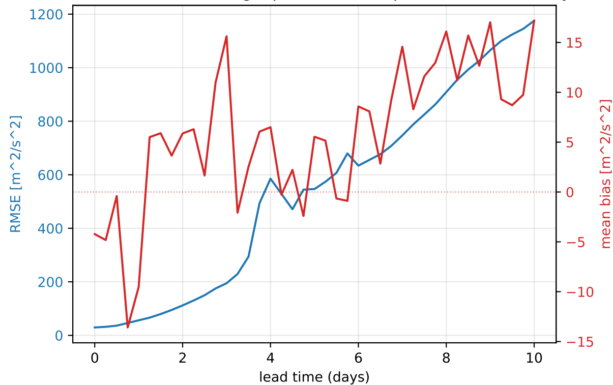
NextGEMS-2049 — 500 hPa geopotential (europe, mean of 355 daily inits)
