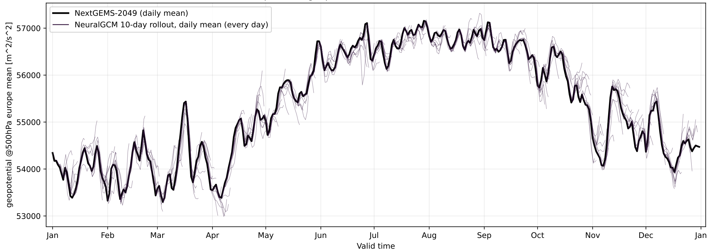
Europe-mean geopotential at 500 hPa — NextGEMS-2049
