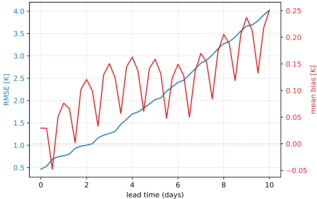
NextGEMS-2049 — 950 hPa temperature (europe, mean of 355 daily inits)
