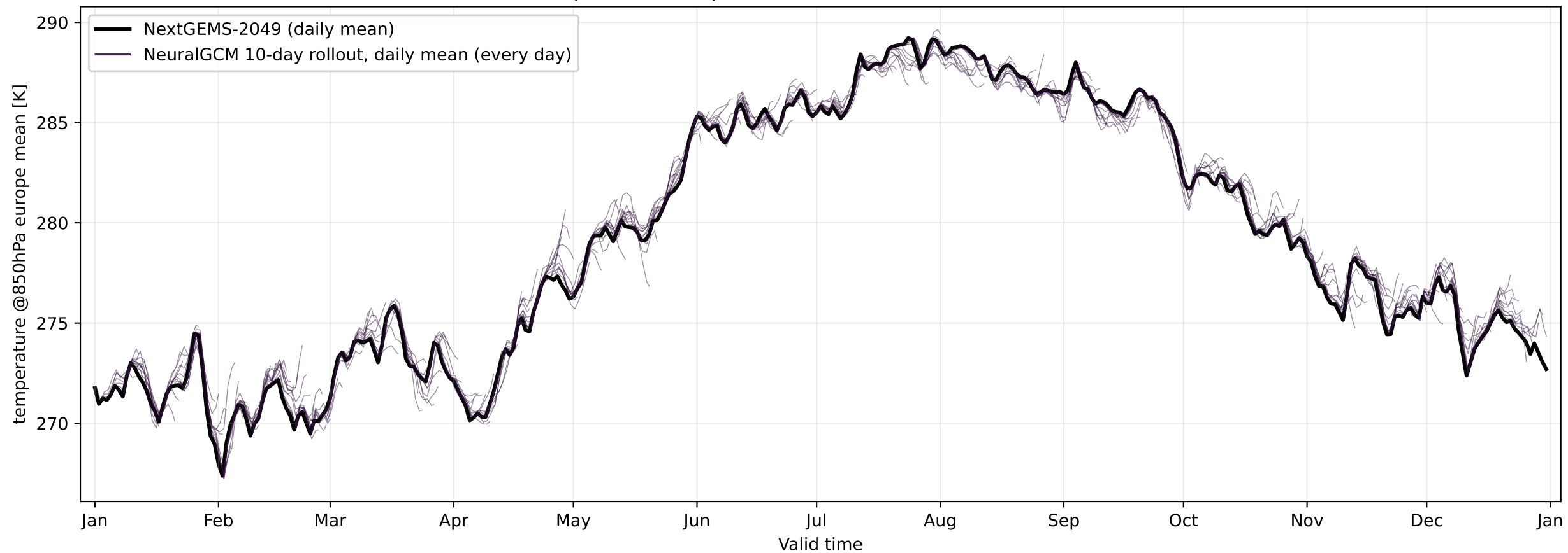
Europe-mean temperature at 850 hPa — NextGEMS-2049
