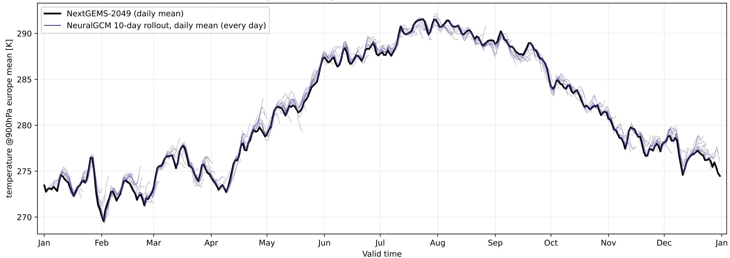
Europe-mean temperature at 900 hPa — NextGEMS-2049
