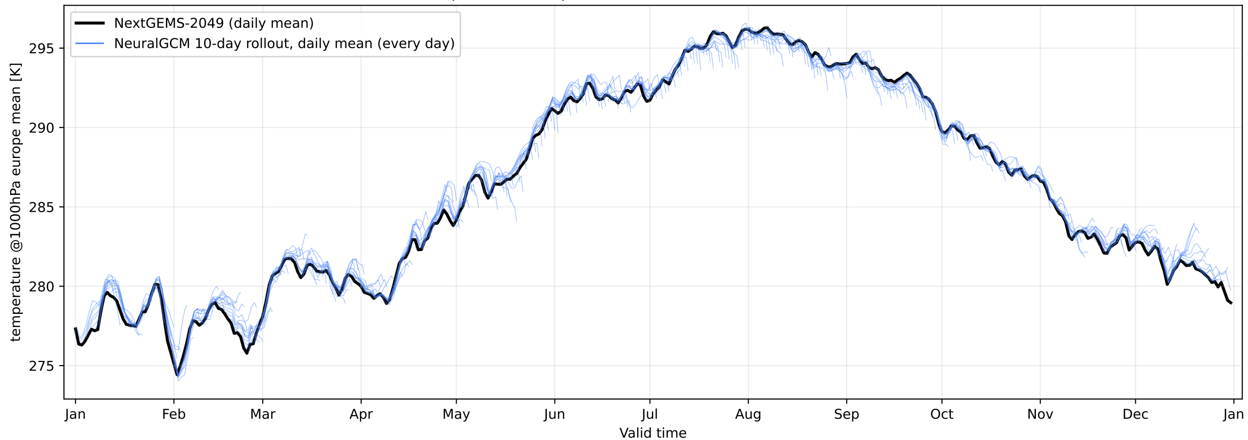
Europe-mean temperature at 1000 hPa — NextGEMS-2049
