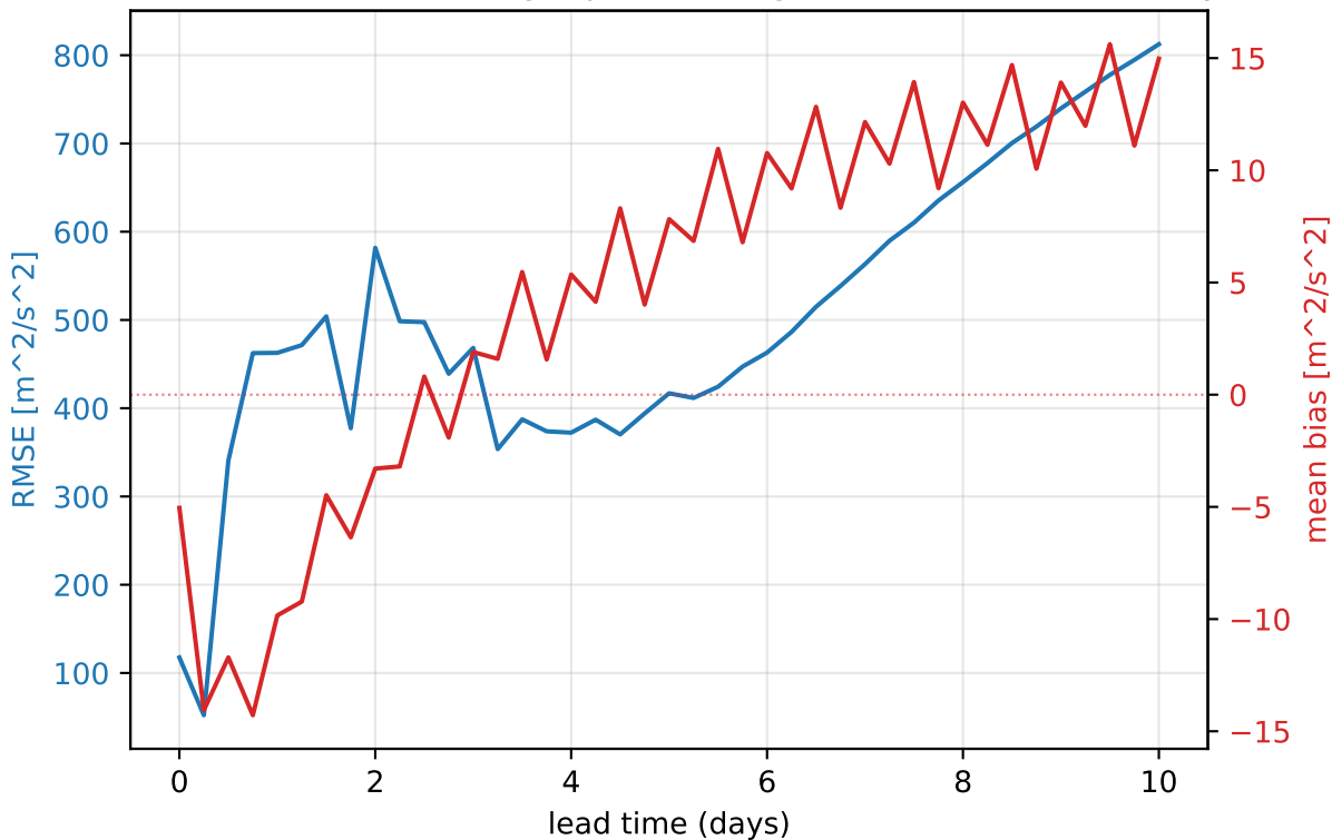
NextGEMS-2049 — 500 hPa geopotential (global, mean of 355 daily inits)
