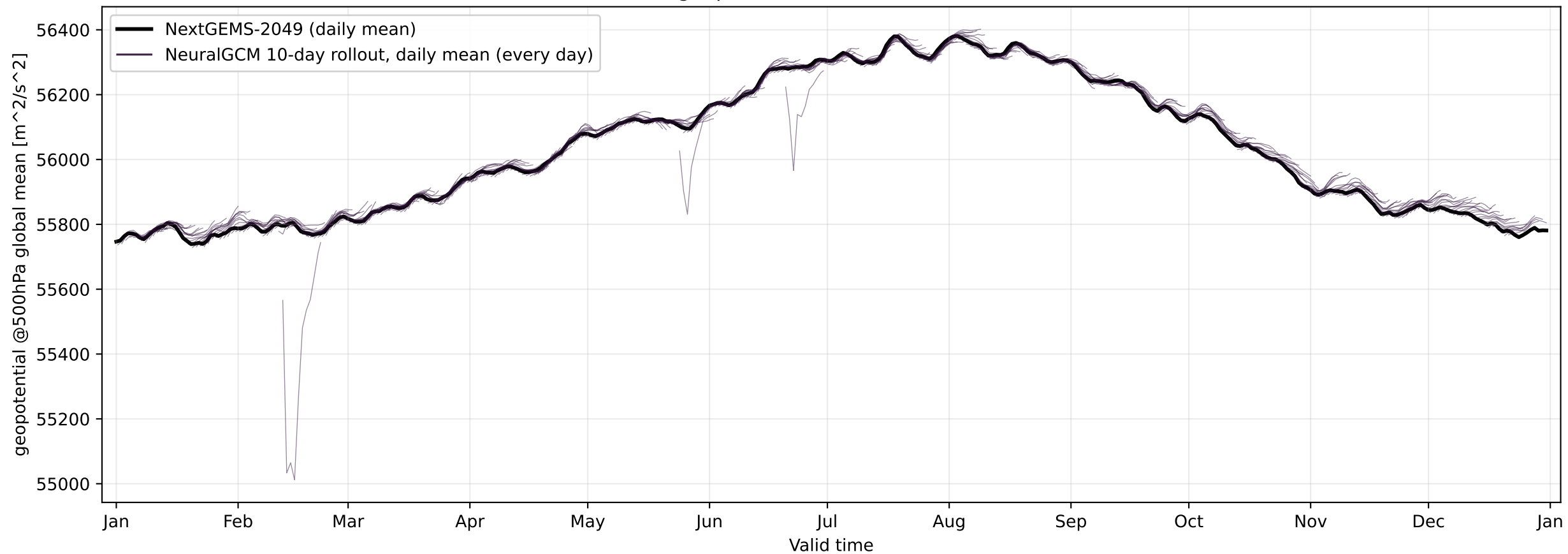
Global-mean geopotential at 500 hPa — NextGEMS-2049
