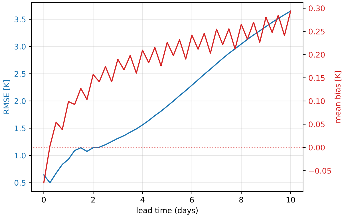
NextGEMS-2049 — 850 hPa temperature (global, mean of 355 daily inits)
