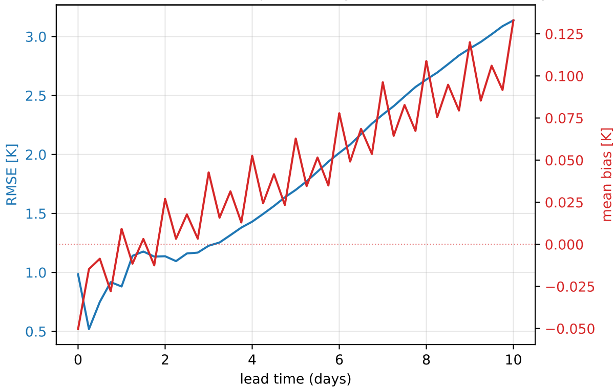
NextGEMS-2049 — 950 hPa temperature (global, mean of 355 daily inits)
