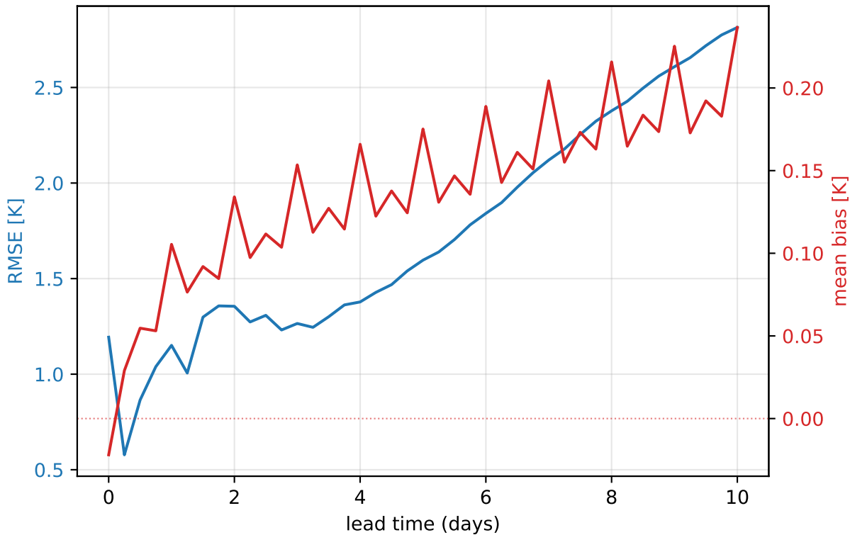
NextGEMS-2049 — 1000 hPa temperature (global, mean of 355 daily inits)
