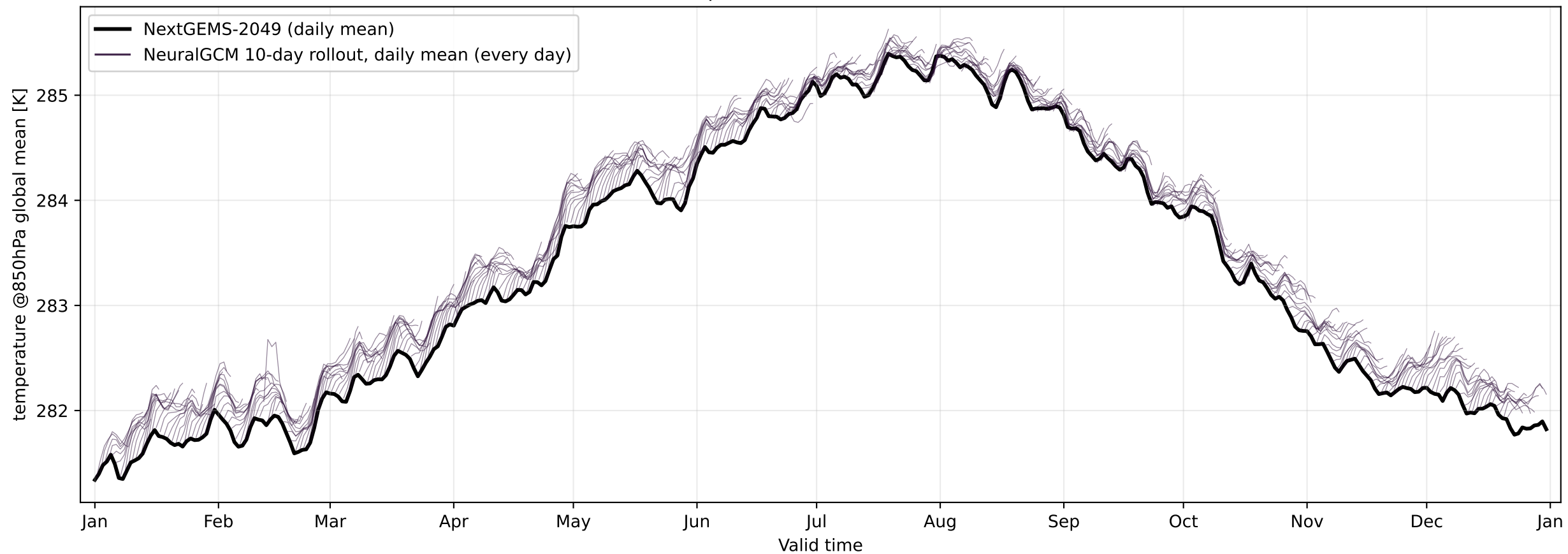
Global-mean temperature at 850 hPa — NextGEMS-2049
