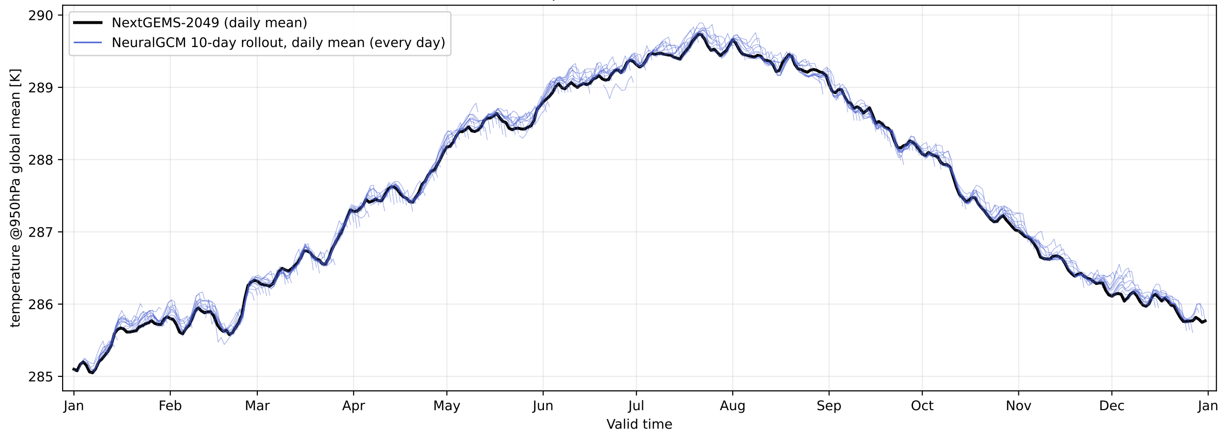
Global-mean temperature at 950 hPa — NextGEMS-2049
