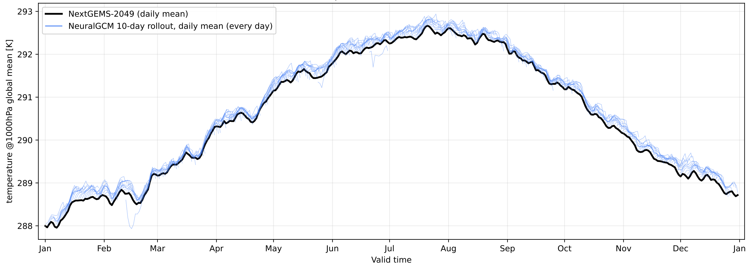
Global-mean temperature at 1000 hPa — NextGEMS-2049
