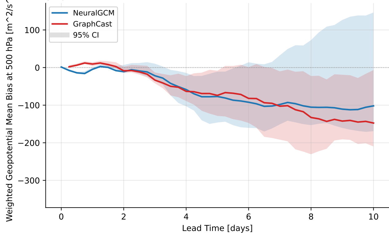
geopotential@500 hPa — mean bias over the 6 2023 cordex heat waves (6 events, > p99)
