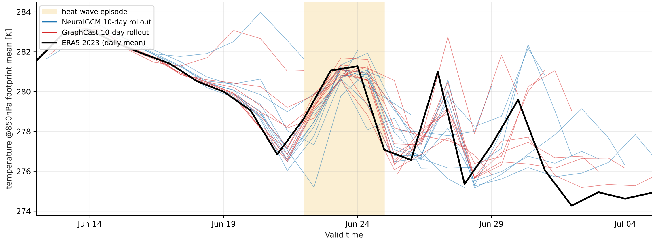
Europe heat-wave 2023-06-22..2023-06-25 — footprint-mean temperature @ 850 hPa (cortex, > p99)
